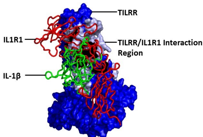
Predictive 3D- model of the IL1R1/TILRR complex
